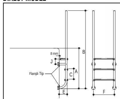
DIRECT MODEL
