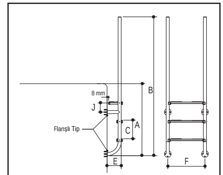
DIRECT MODEL
